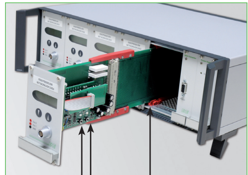
push-buttons for humidity / temperature calibration
